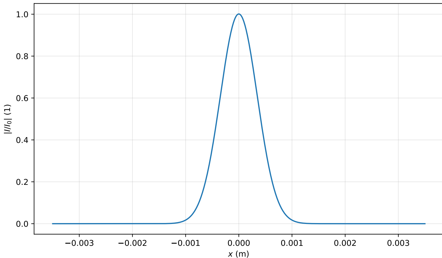
Intensity profile I(x, y = 0, z = 0.159m)/I_0 , P_{in}=0.3P_{cr} , artificial time
